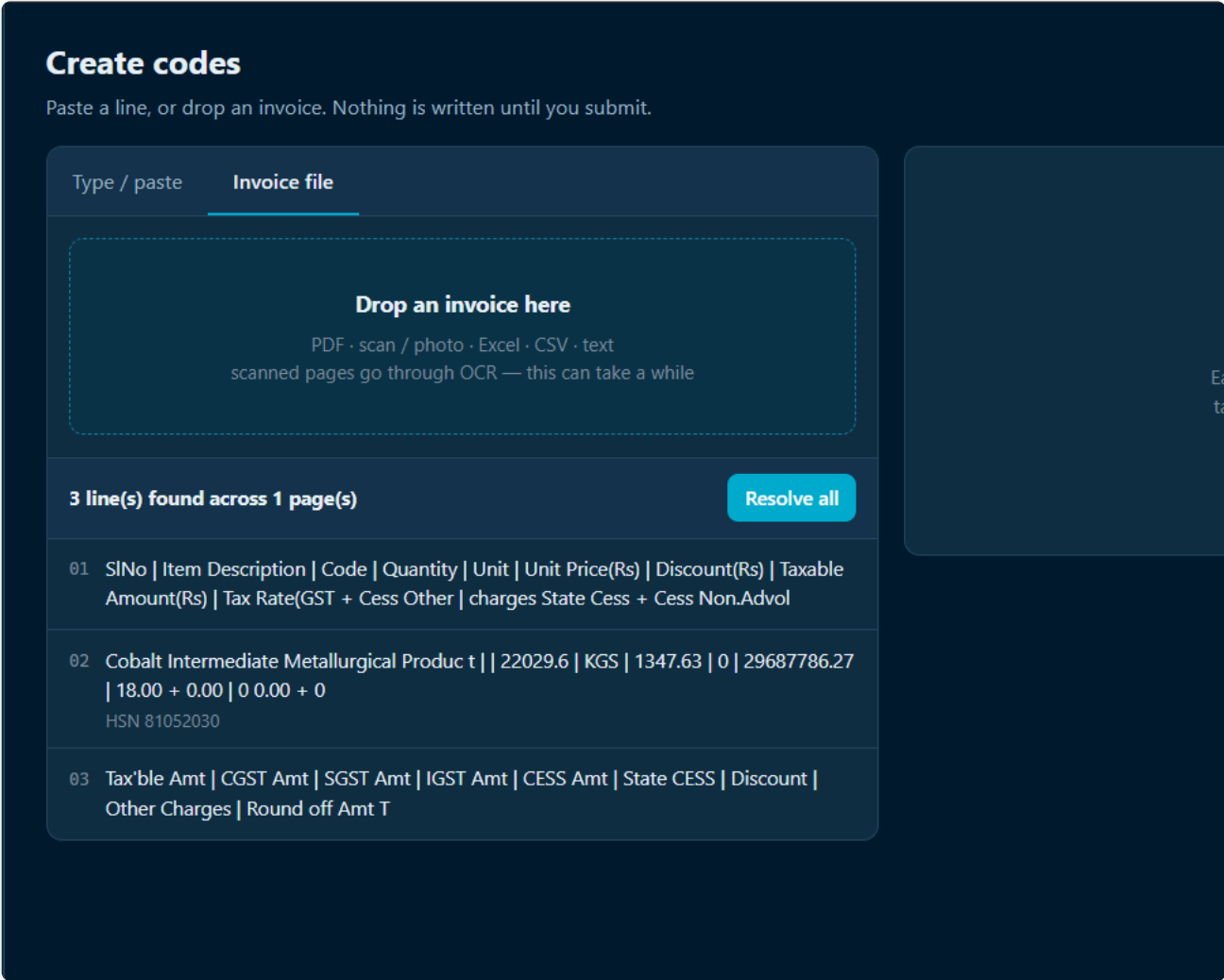
OCR-parsed invoice lines ready for code generation
